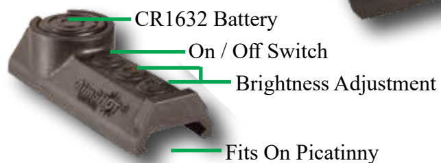
Wireless Remote
